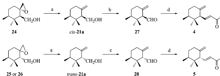
Scheme 7. a) [\text{Bu}_3\text{SnAlMe}_3]\text{Li} , \text{CH}_2\text{Cl}_2 , 0^\circ\text{C} , 2 h, 70% yield; b) Swern oxidation, 86% yield; c) Dess–Martin periodinane reagent, [23] \text{CH}_2\text{Cl}_2 , room temp., 2 h, 96% yield; d) (\text{EtO})_2\text{POCH}_2\text{COCH}_3 , \text{Ba}(\text{OH})_2 \cdot 8\text{H}_2\text{O} , \text{THF}/\text{H}_2\text{O} = 40:1 , room temp., 18 h; 4 70% yield, 5 72% yield
