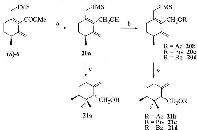
Scheme 5. a) DIBALH, Et 2 O, 0 °C, 1 h, 85% yield; b) RCOCl, pyridine, cat. DMAP, CH 2 Cl 2 , 1 h, 85% ( 20b ), 98% ( 20c ), 99% ( 20d ); c) Hg(OCOCF 3 ) 2 , CH 3 CH 2 CN, –78 °C, 45 min; then satd. aq. NaCl, 0 °C, 30 min; then NaBH 4 , NaOH 15%, 0 °C, 30 min
