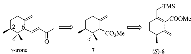
Scheme 1. Retrosynthesis of \gamma -irone
