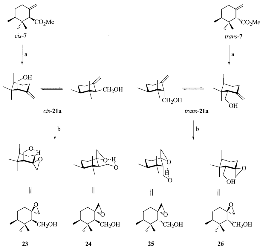
Scheme 6. a) DIBALH, Et 2 O, 0 ^{\circ}\text{C} , 45 min, 92% yield; b) t BuOOH, VO(acac) 2 , CH 2 Cl 2 , -20^{\circ}\text{C} , 22 h; 85% isolated yield of compounds 24–26 in a ratio of 56:38:6, < 2% (GC) of compound 23
