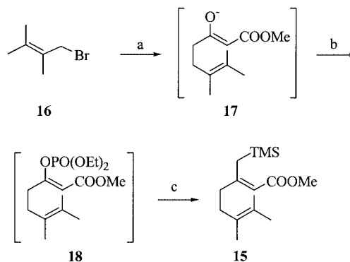
Scheme 3. a) Na/Li methyl acetoacetate dianion, THF, 0 °C to room temp., 1 h; b) ClP(O)(OEt) 2 , 0 °C to room temp., 1.5 h; c) Me 3 SiCH 2 MgCl, cat. Ni(acac) 2 , THF, 0 °C, 1 h, 42% yield (3 steps)
