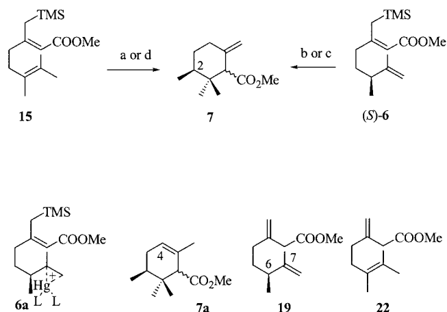
Scheme 4. a) SnCl 4 , wet CH 2 Cl 2 , −30 to −20 °C, 2 h, 85% yield; b) SnCl 4 , wet CH 2 Cl 2 , −30 to −20 °C, 1 h, 92% yield or TiCl 4 , dry CH 2 Cl 2 , −30 to −20 °C, 1 h, 87% yield; c) Hg(OCOCF 3 ) 2 , CH 3 CN, 0 °C, 45 min; then satd. aq. NaCl, 0 °C, 30 min; then NaBH 4 , NaOH 15%, 0 °C, 30 min, 82% yield; d) Hg(OCOCF 3 ) 2 , CH 3 CN, −40 °C, 45 min; then satd. aq. NaCl, 0 °C, 30 min; then NaBH 4 , NaOH 15%, 0 °C, 30 min, 57% yield
