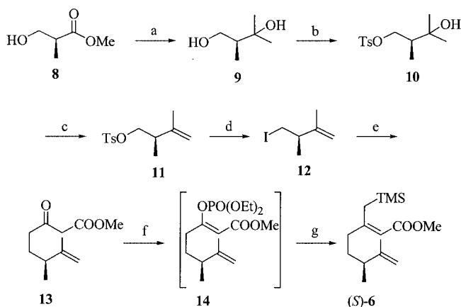
Scheme 2. a) MeMgBr, Et 2 O, 0 °C, 1.5 h; b) TsCl, pyridine, 0 °C, 15 h; c) CH 3 SO 2 Cl, Et 3 N, Et 2 O, 0 °C to room temp., 15 h, 66% yield (3 steps); d) LiI, THF, reflux, 2 h; e) Na/Li methyl acetoacetate dianion, THF, 0 °C to room temp., 1.5 h, 40% yield (2 steps, unoptimized); f) NaH, THF, 0 °C, 15 min, then ClP(O)(OEt) 2 , 0 °C to room temp., 1.5 h; g) Me 3 SiCH 2 MgCl (1 M in THF), cat. Ni(acac) 2 , 0 °C, 1 h, 69% yield (2 steps)
