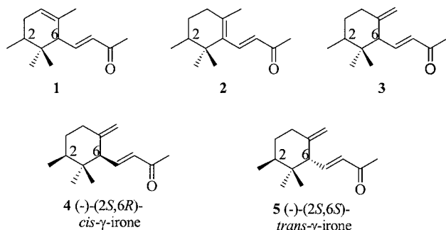
Figure 1. Components of Iris oil
